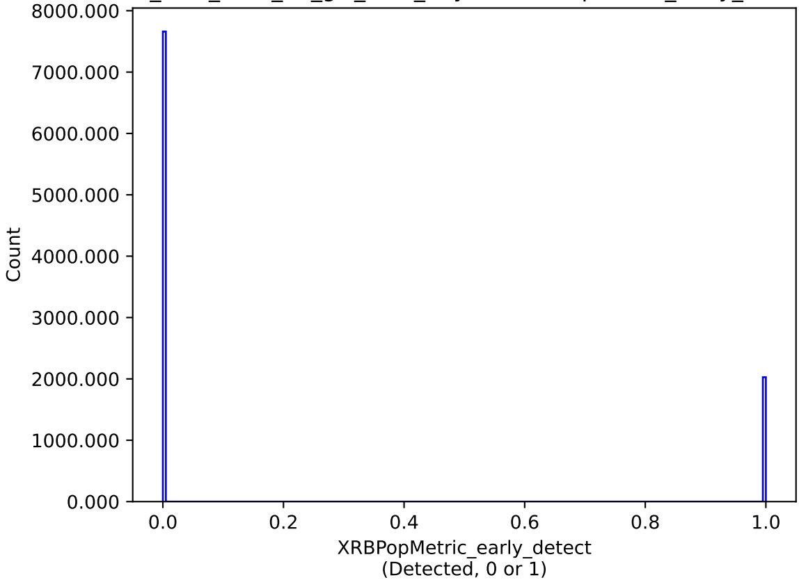
too_elab_r128_d3_giz_v3.4_10yrs : XRBPopMetric_early_detect
