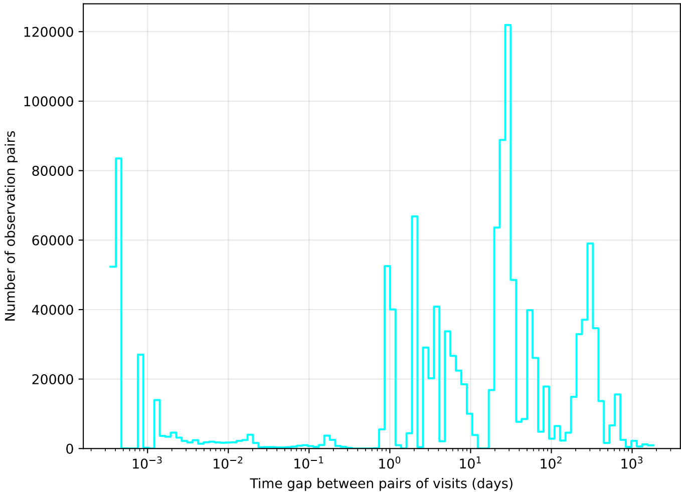
too_elab_r128_d3_giz_v3.4_10yrs u band: Tgaps observationStartMJD
