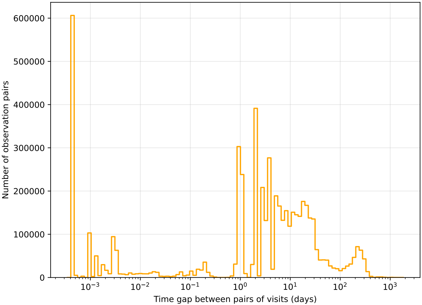
too_elab_r128_d3_giz_v3.4_10yrs r band: Tgaps observationStartMJD
