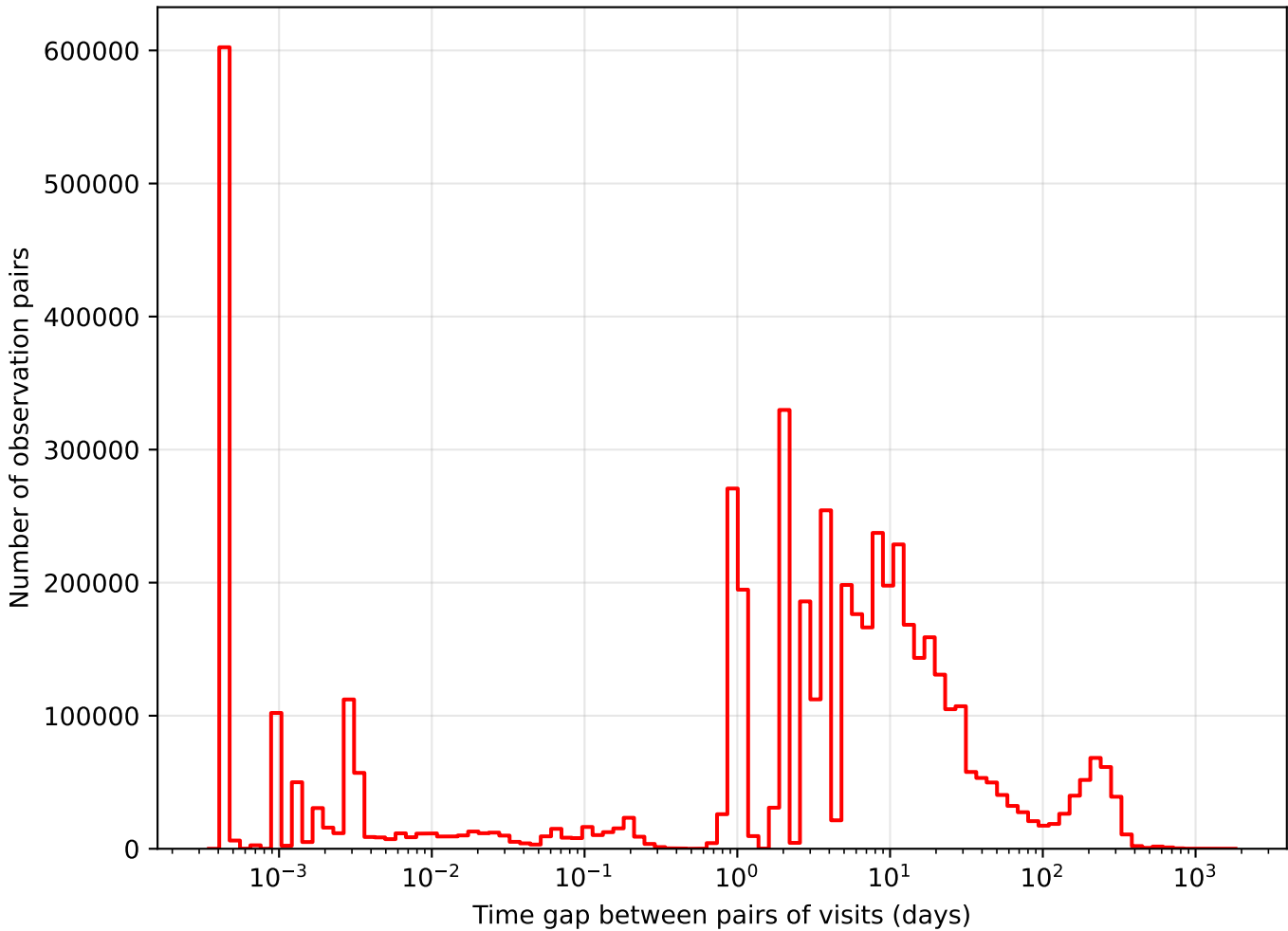
too_elab_r128_d3_giz_v3.4_10yrs i band: Tgaps observationStartMJD
