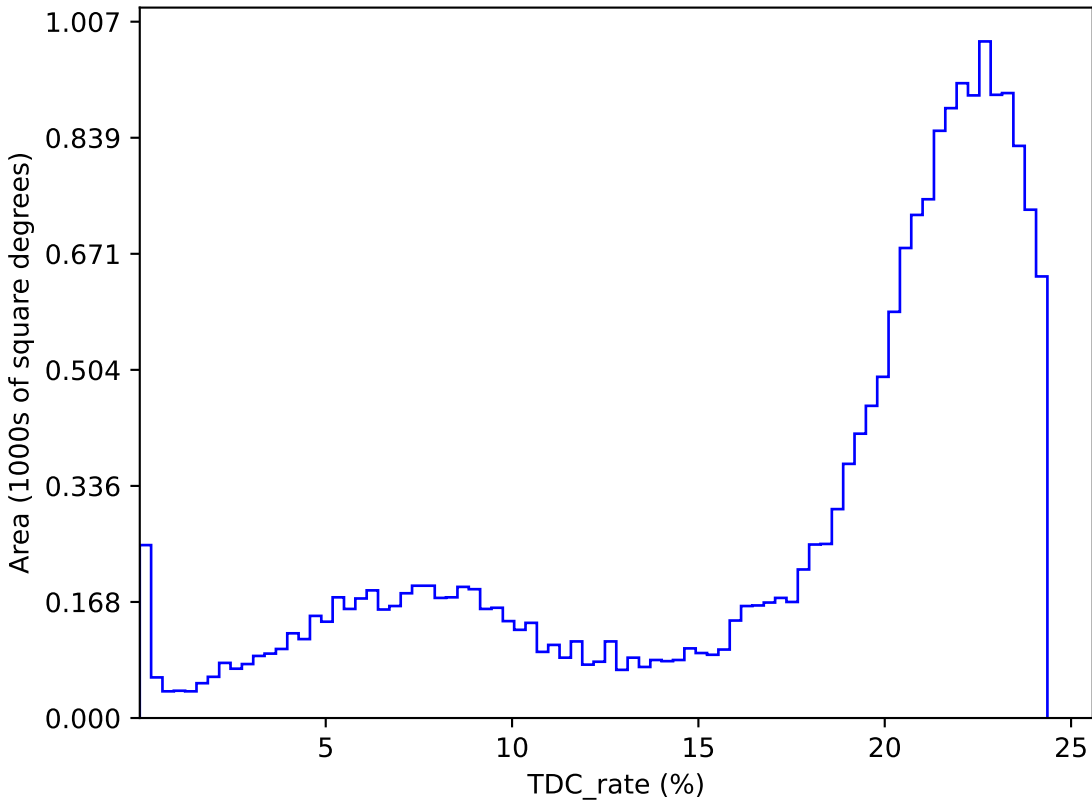
too_elab_r128_d3_giz_v3.4_10yrs : TDC_rate
