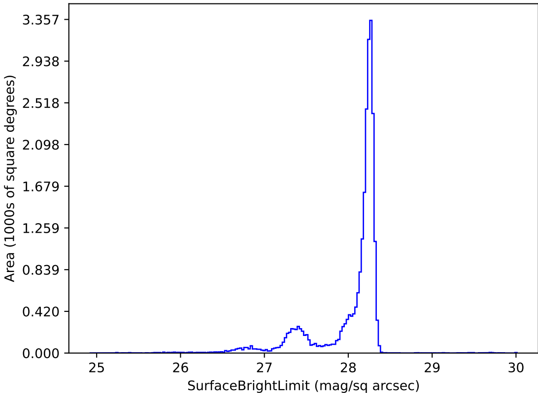
too_elab_r128_d3_giz_v3.4_10yrs y: SurfaceBrightLimit
