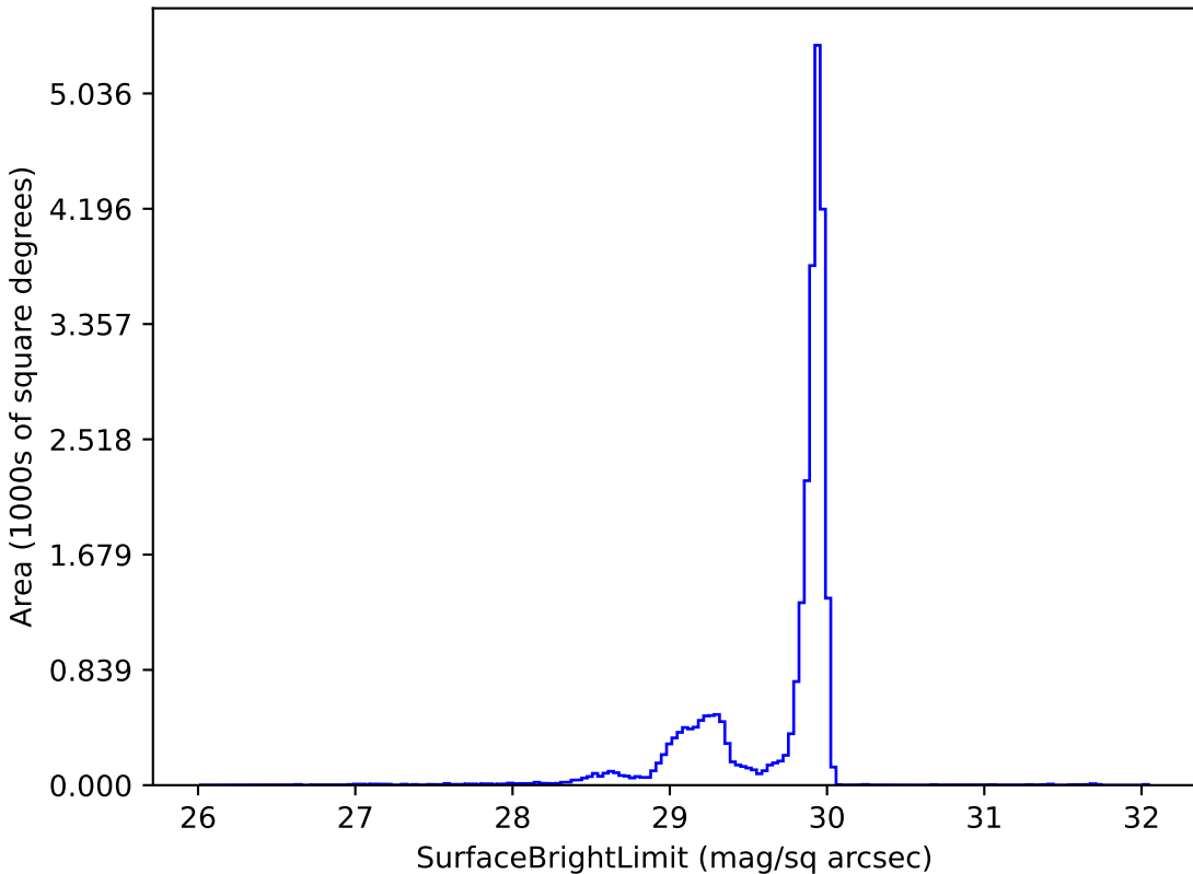
too_elab_r128_d3_giz_v3.4_10yrs i: SurfaceBrightLimit
