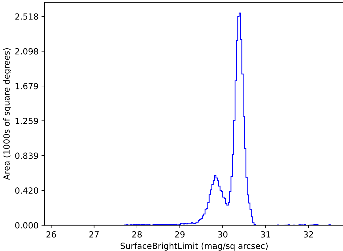
too_elab_r128_d3_giz_v3.4_10yrs g: SurfaceBrightLimit
