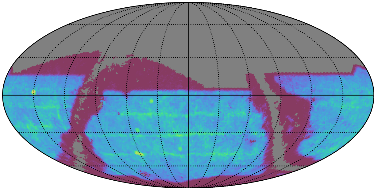
too_elab_r128_d3_giz_v3.4_10yrs : SNSLMetric
