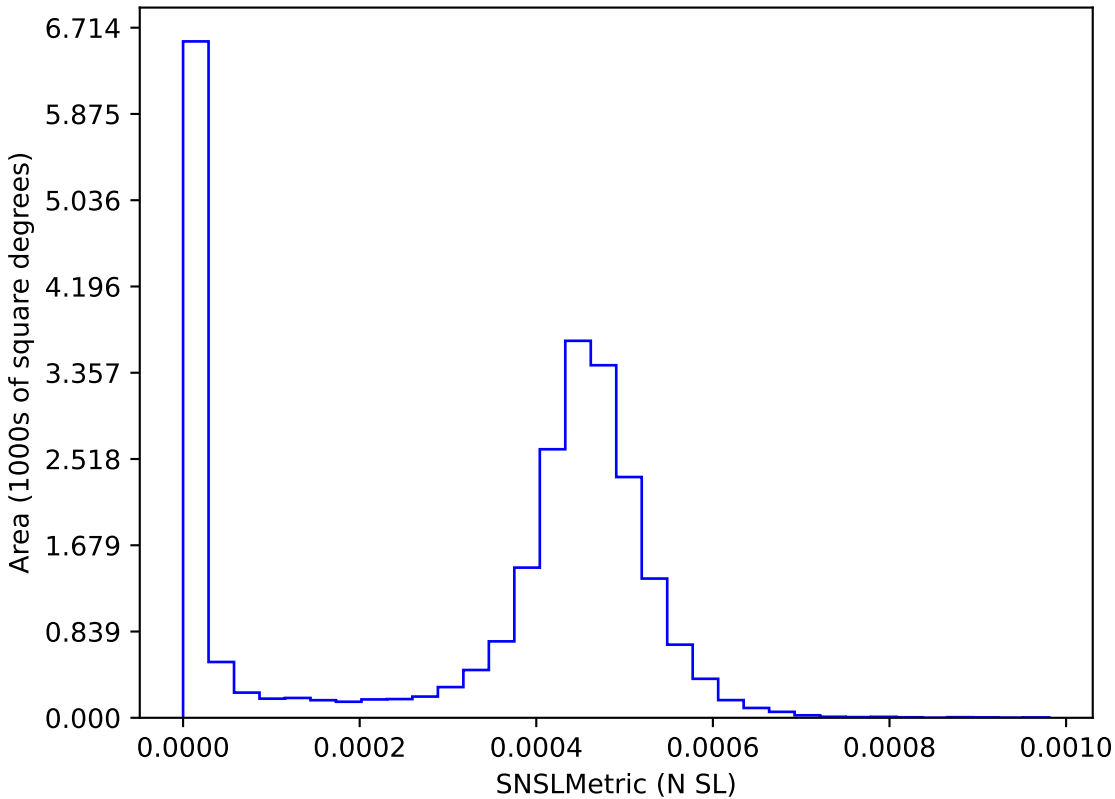
too_elab_r128_d3_giz_v3.4_10yrs : SNSLMetric
