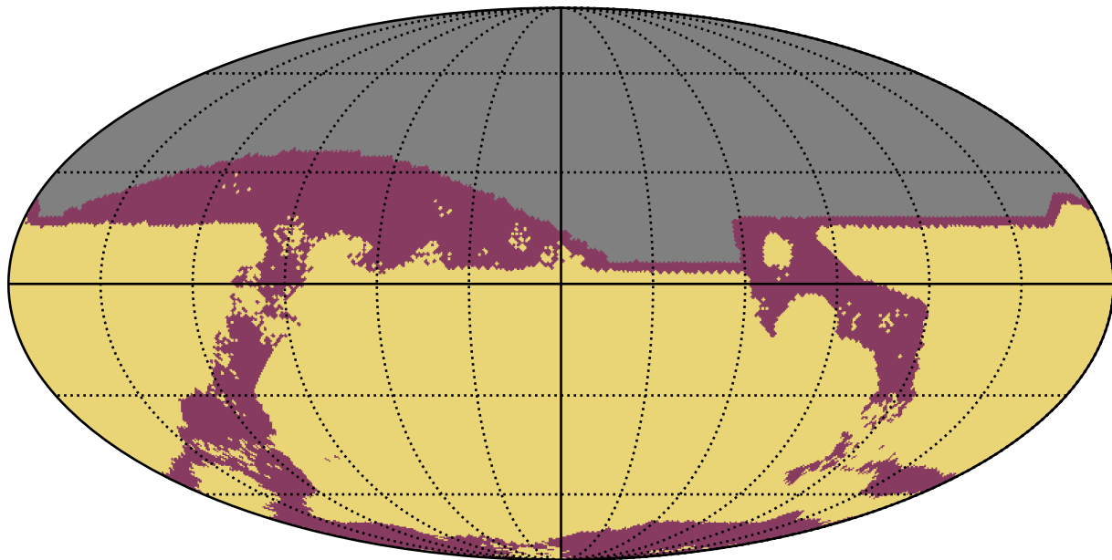
too_elab_r128_d3_giz_v3.4_10yrs : RapidRevisits
