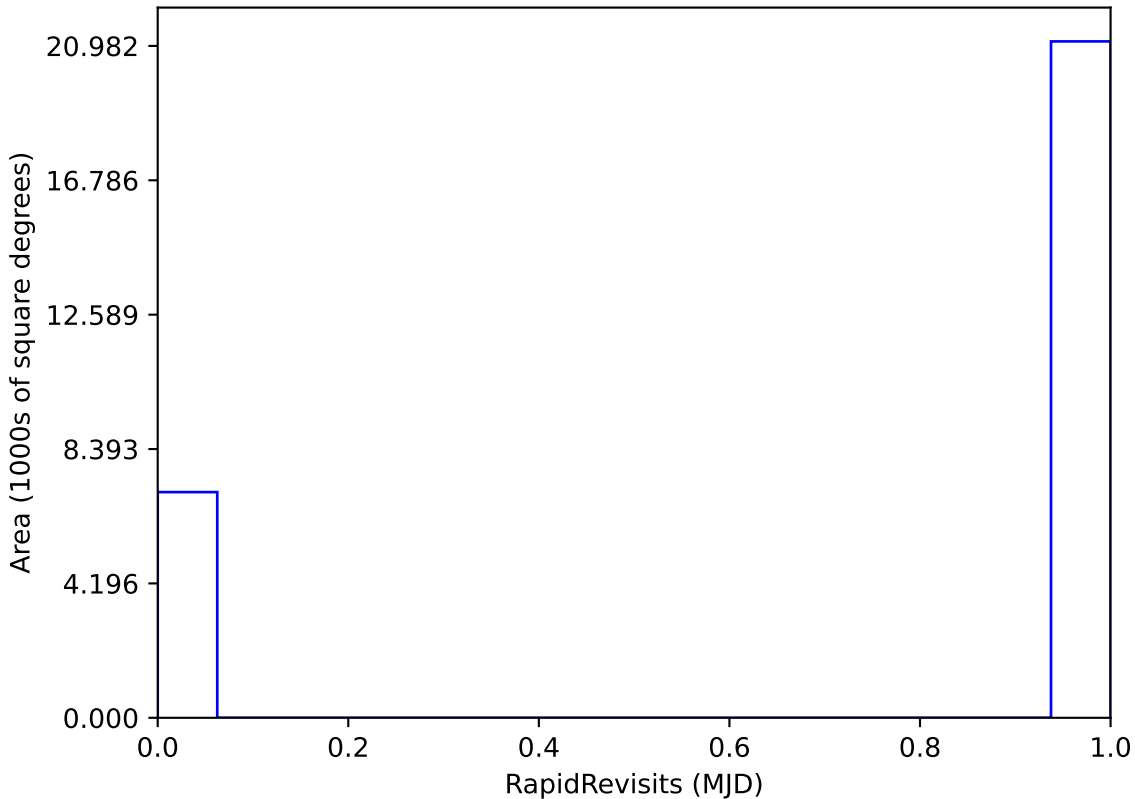
too_elab_r128_d3_giz_v3.4_10yrs : RapidRevisits
