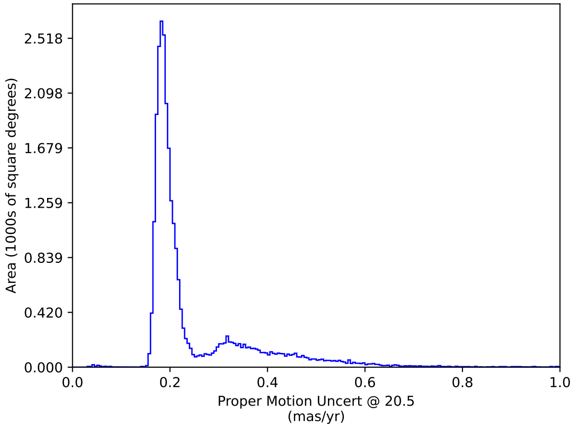
too_elab_r128_d3_giz_v3.4_10yrs : Proper Motion Uncert @ 20.5
