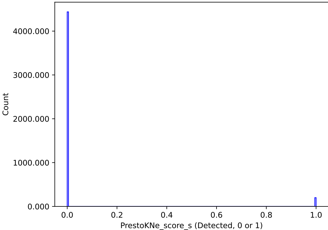
too_elab_r128_d3_giz_v3.4_10yrs : PrestoKNe_score_s
