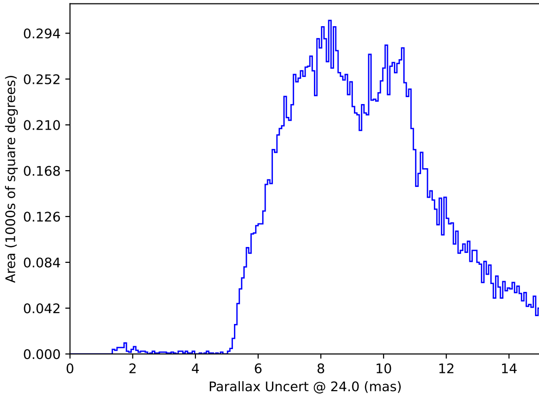
too_elab_r128_d3_giz_v3.4_10yrs : Parallax Uncert @ 24.0
