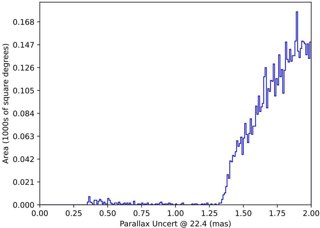
too_elab_r128_d3_giz_v3.4_10yrs : Parallax Uncert @ 22.4
