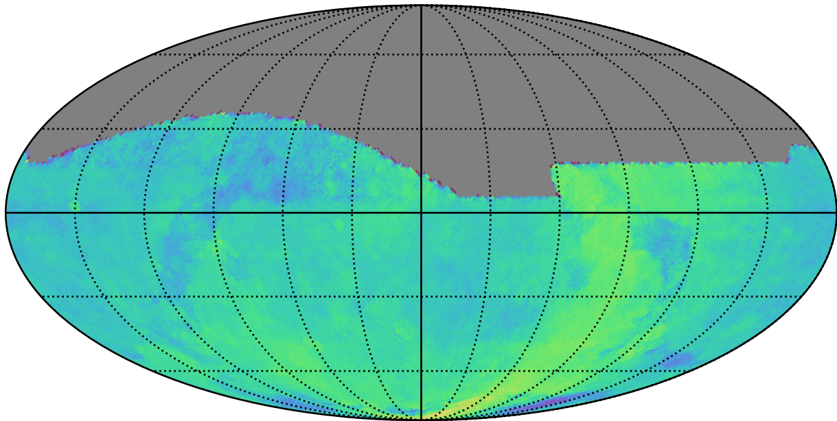
too_elab_r128_d3_giz_v3.4_10yrs : Parallax Coverage @ 22.4
