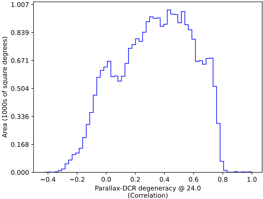
too_elab_r128_d3_giz_v3.4_10yrs : Parallax-DCR degeneracy @ 24.0
