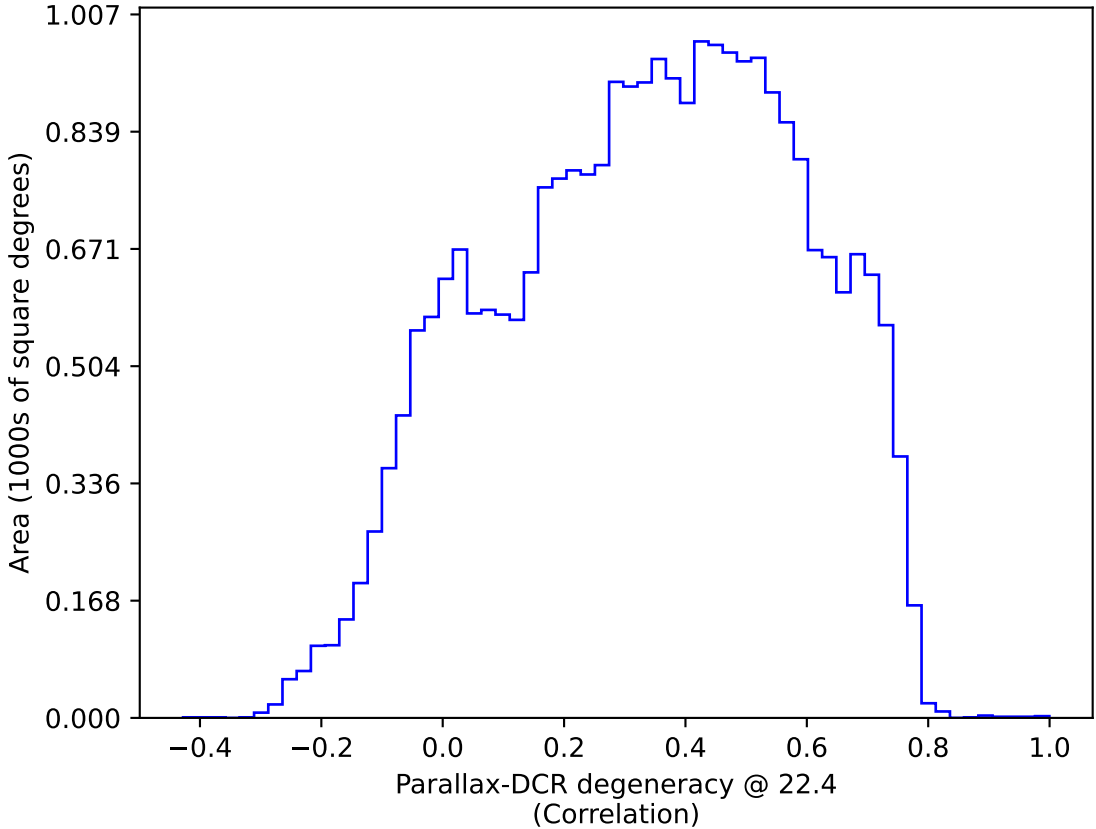
too_elab_r128_d3_giz_v3.4_10yrs : Parallax-DCR degeneracy @ 22.4
