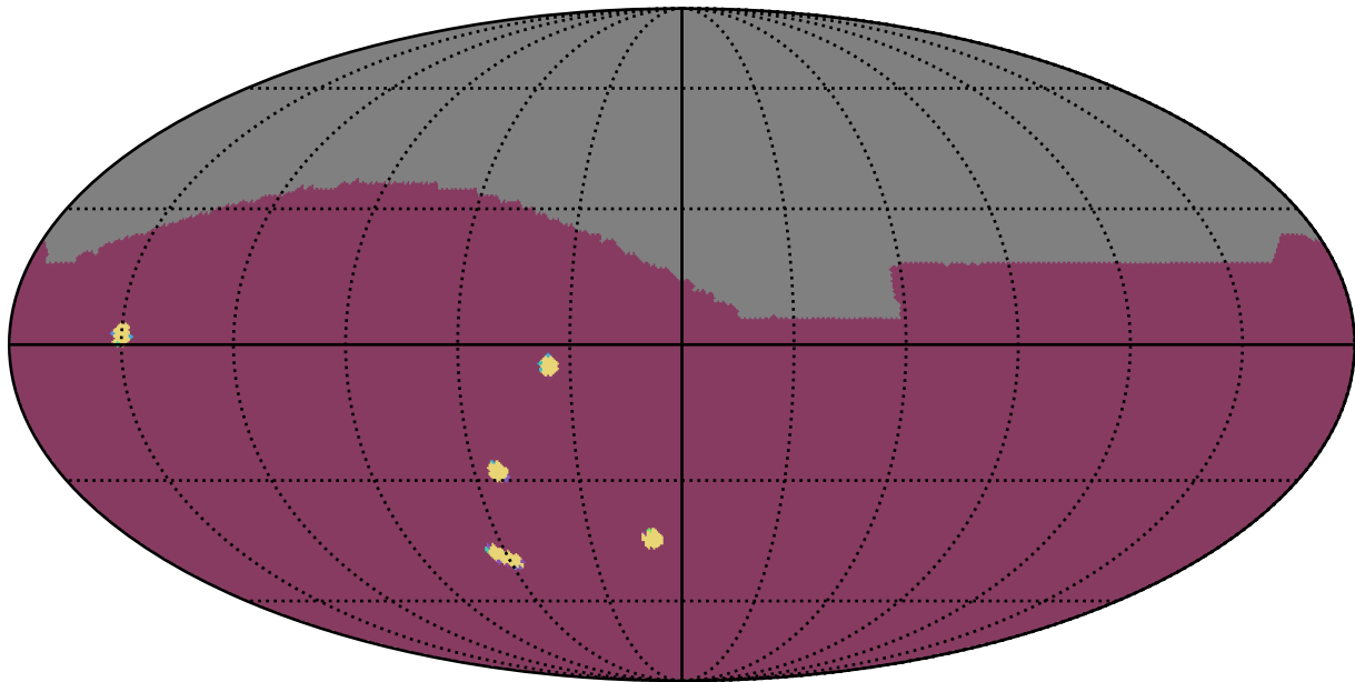
too_elab_r128_d3_giz_v3.4_10yrs : NumberOfQuickRevisits
