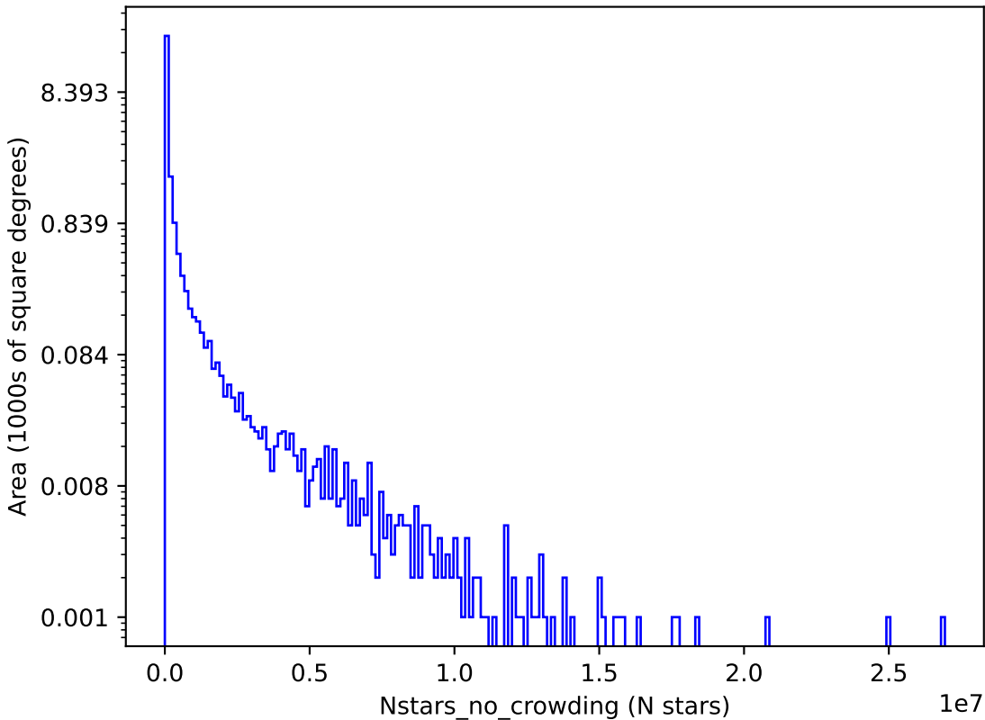
too_elab_r128_d3_giz_v3.4_10yrs i: Nstars_no_crowding
