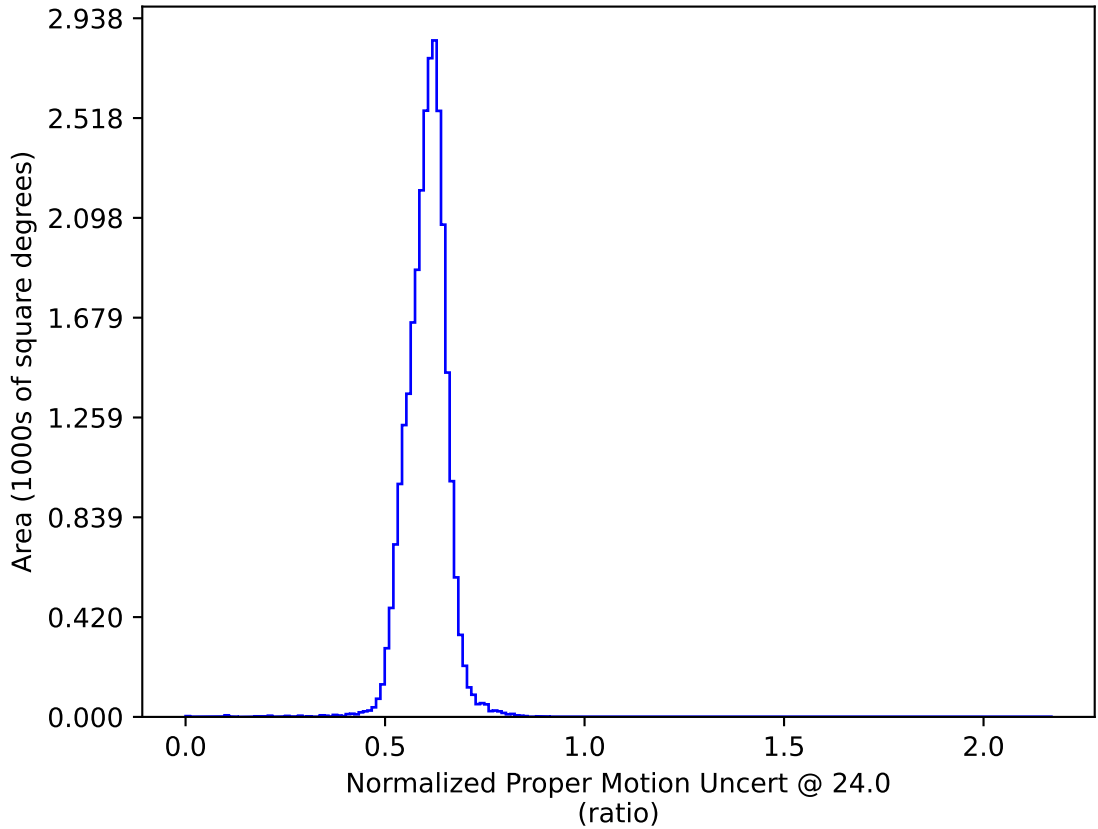
too_elab_r128_d3_giz_v3.4_10yrs : Normalized Proper Motion Uncert @ 24.0
