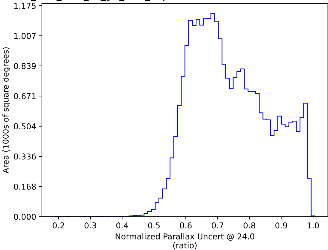
too_elab_r128_d3_giz_v3.4_10yrs : Normalized Parallax Uncert @ 24.0
