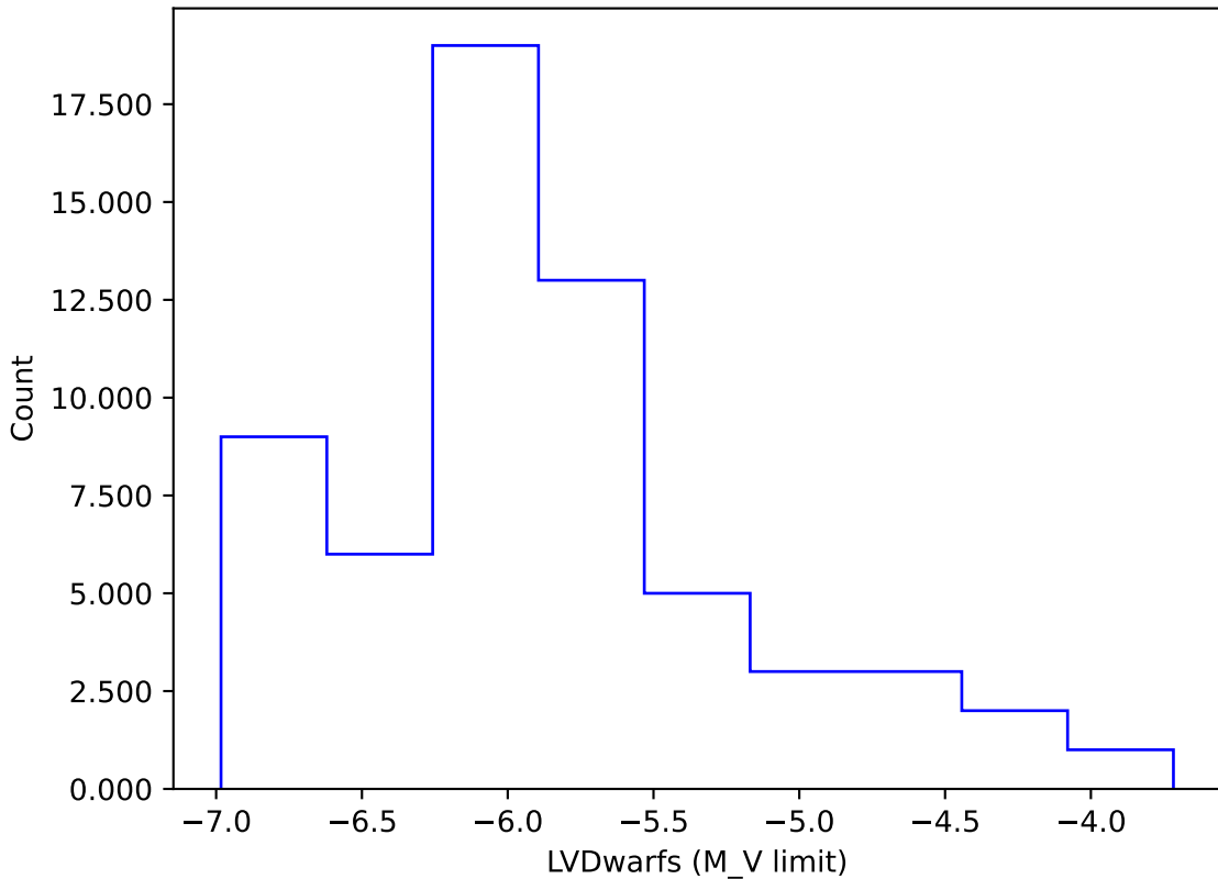
too_elab_r128_d3_giz_v3.4_10yrs gi: LVDwarfs
