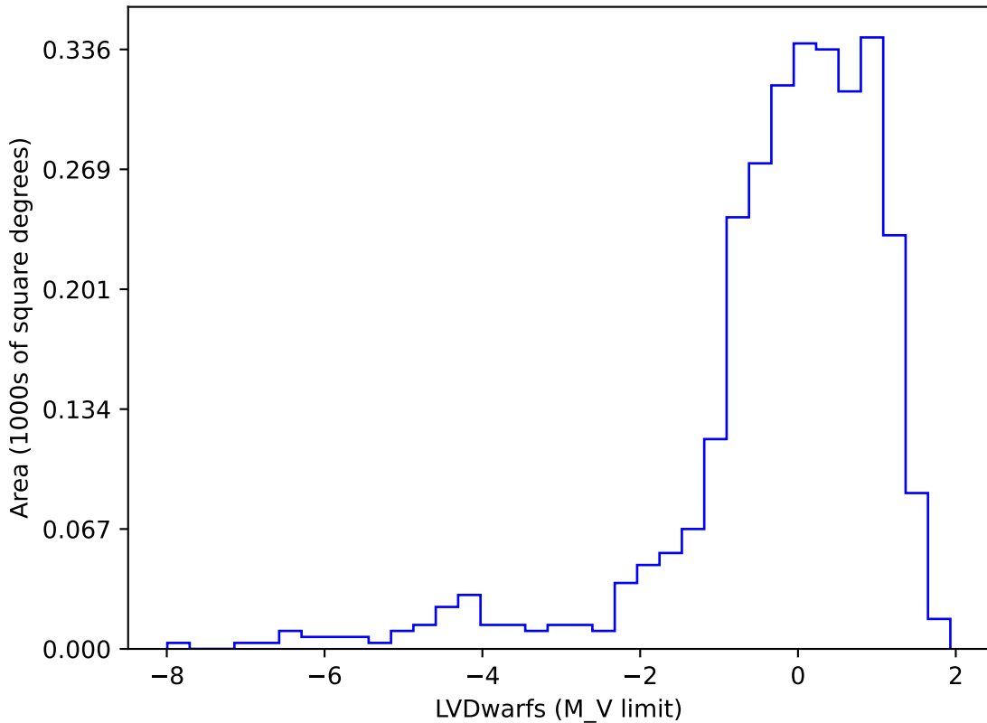
too_elab_r128_d3_giz_v3.4_10yrs gi SCP: LVDwarfs
