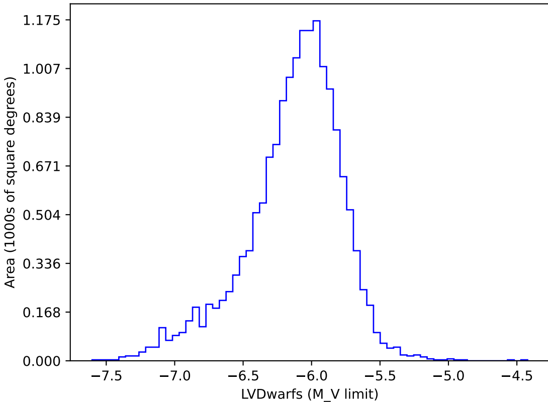
too_elab_r128_d3_giz_v3.4_10yrs gi: LVDwarfs
