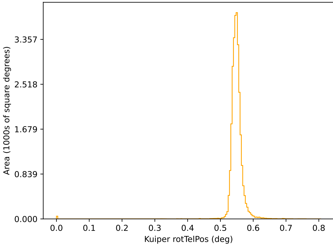
too_elab_r128_d3_giz_v3.4_10yrs r: Kuiper rotTelPos
