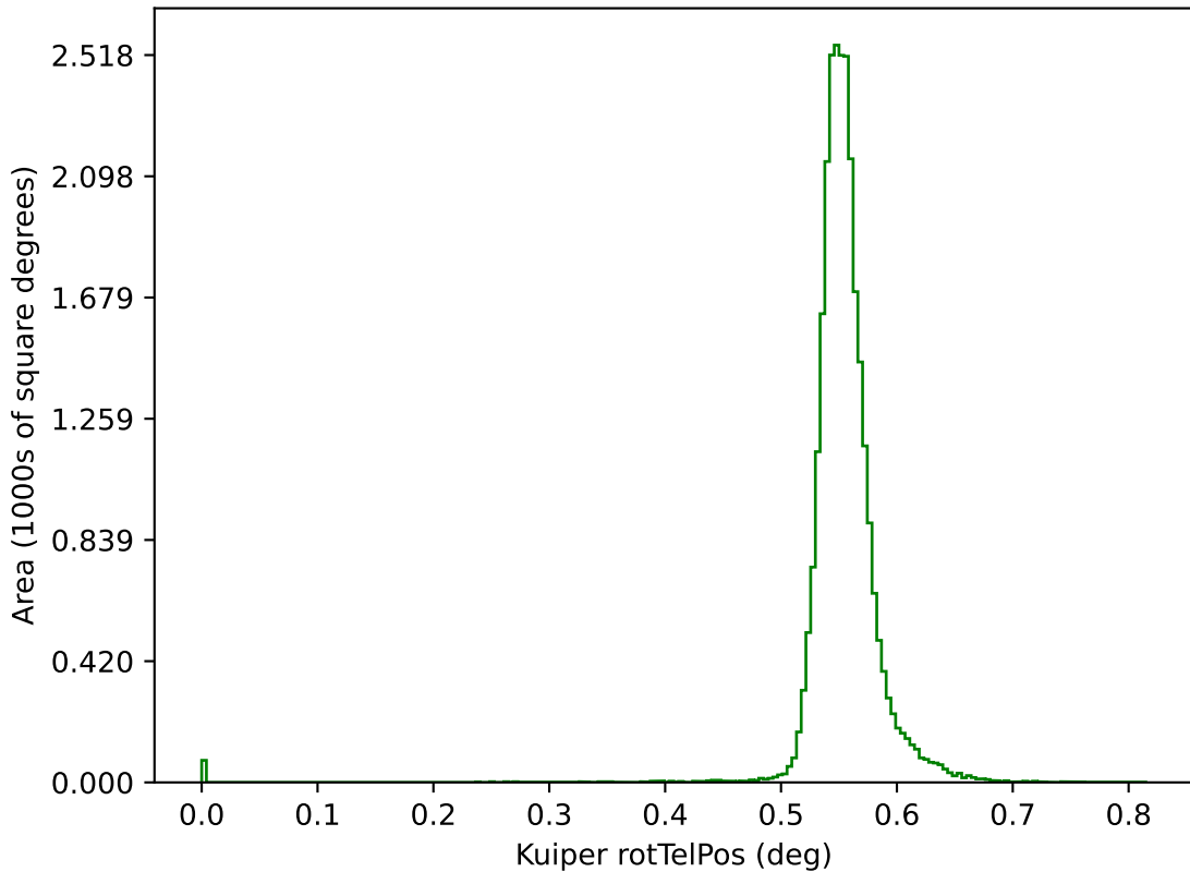
too_elab_r128_d3_giz_v3.4_10yrs g: Kuiper rotTelPos
