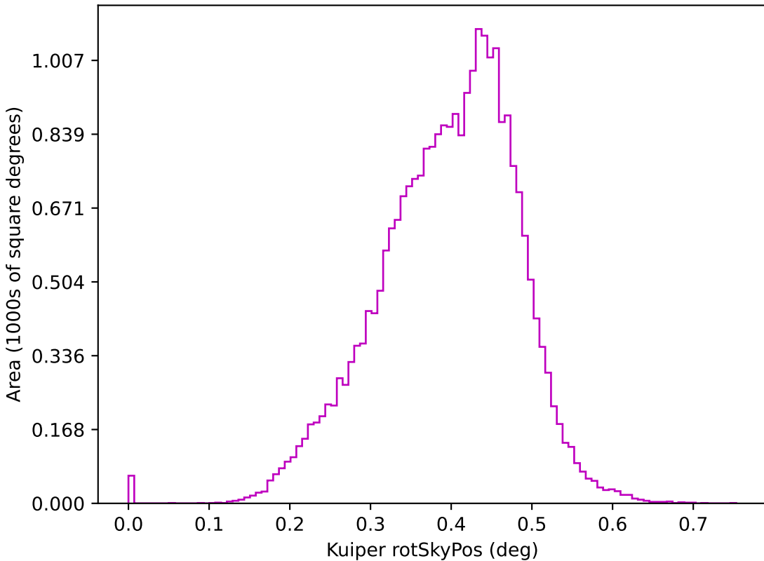
too_elab_r128_d3_giz_v3.4_10yrs z: Kuiper rotSkyPos
