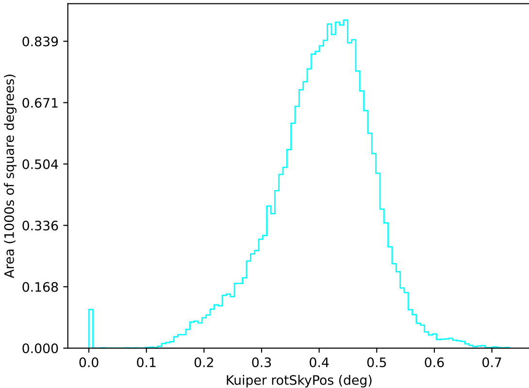
too_elab_r128_d3_giz_v3.4_10yrs u: Kuiper rotSkyPos
