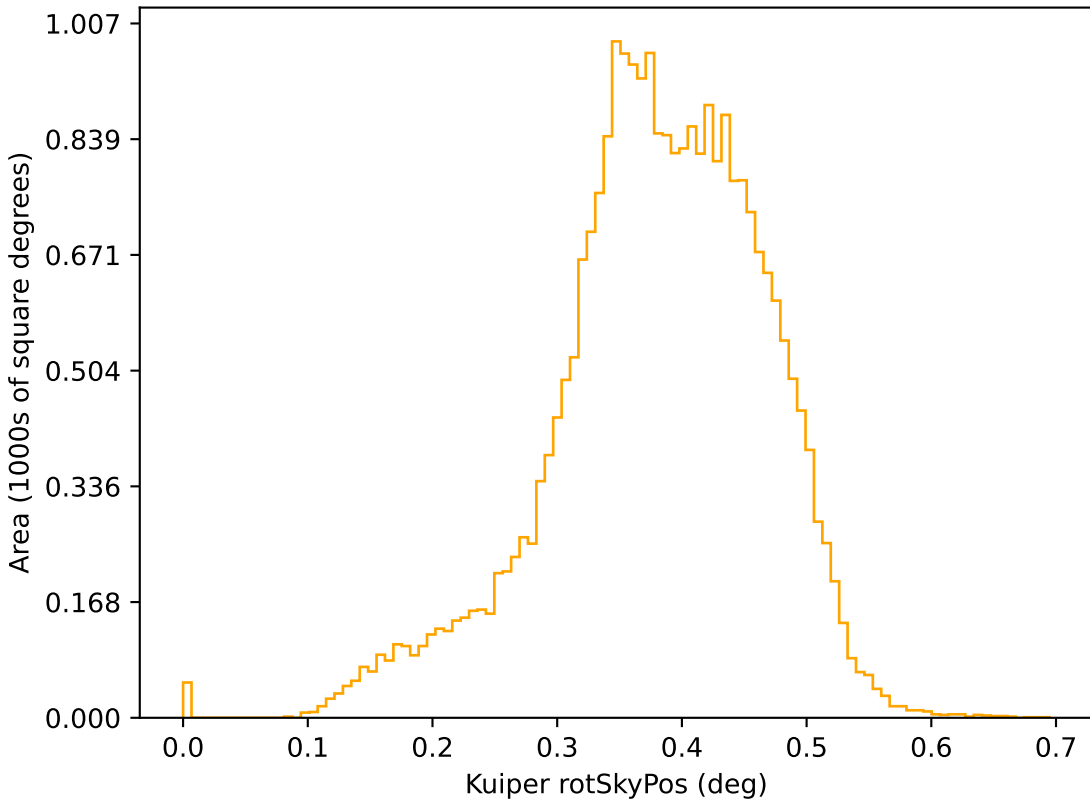
too_elab_r128_d3_giz_v3.4_10yrs r: Kuiper rotSkyPos
