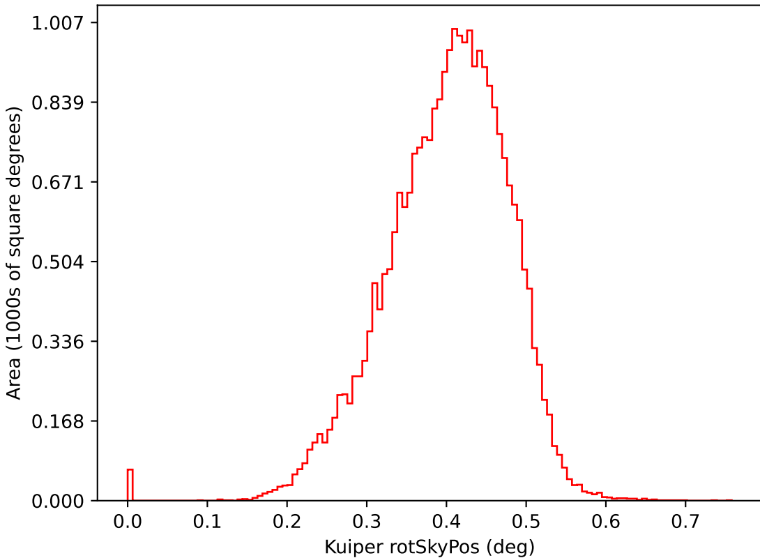
too_elab_r128_d3_giz_v3.4_10yrs i: Kuiper rotSkyPos
