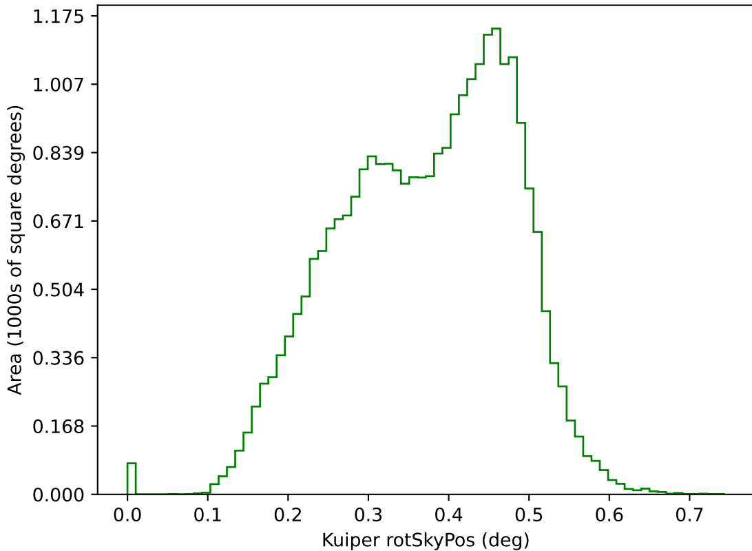
too_elab_r128_d3_giz_v3.4_10yrs g: Kuiper rotSkyPos
