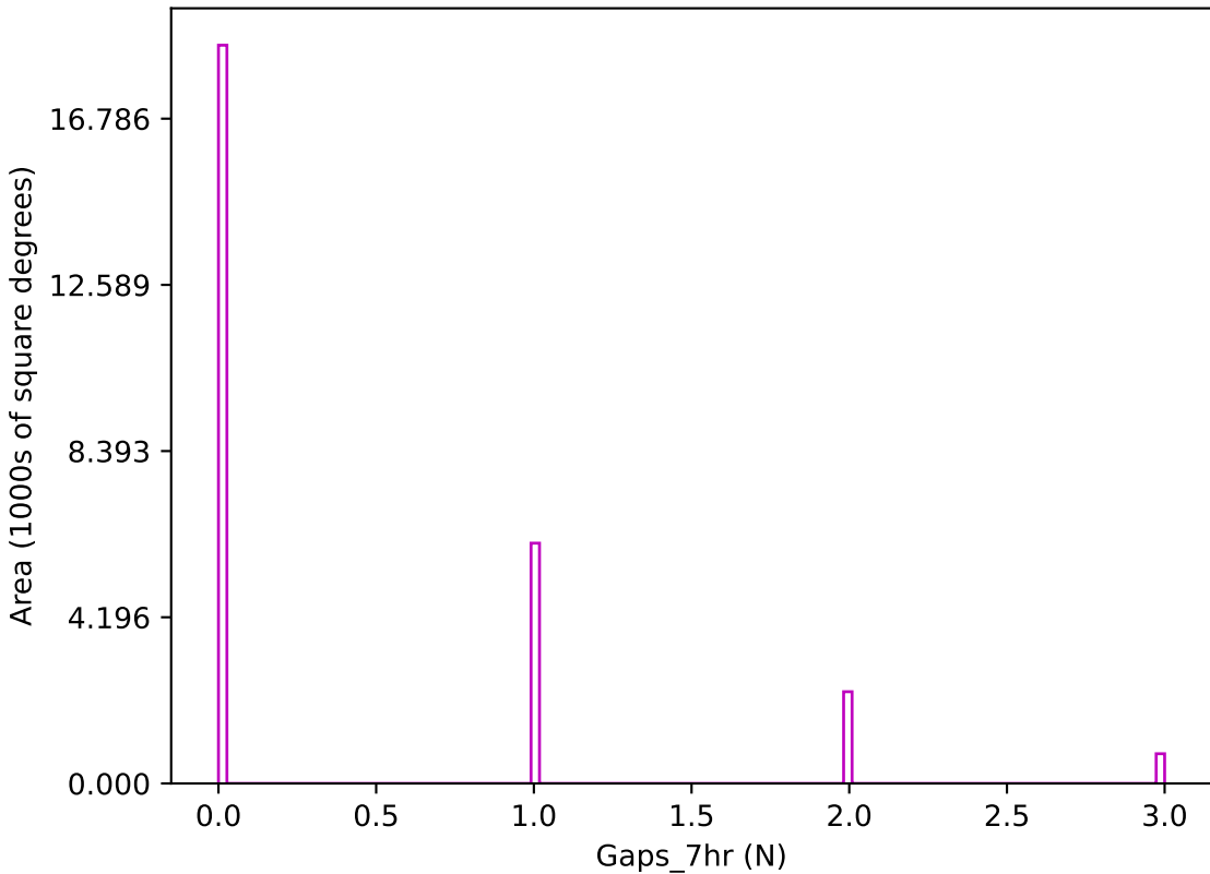
too_elab_r128_d3_giz_v3.4_10yrs z band: Gaps_7hr
