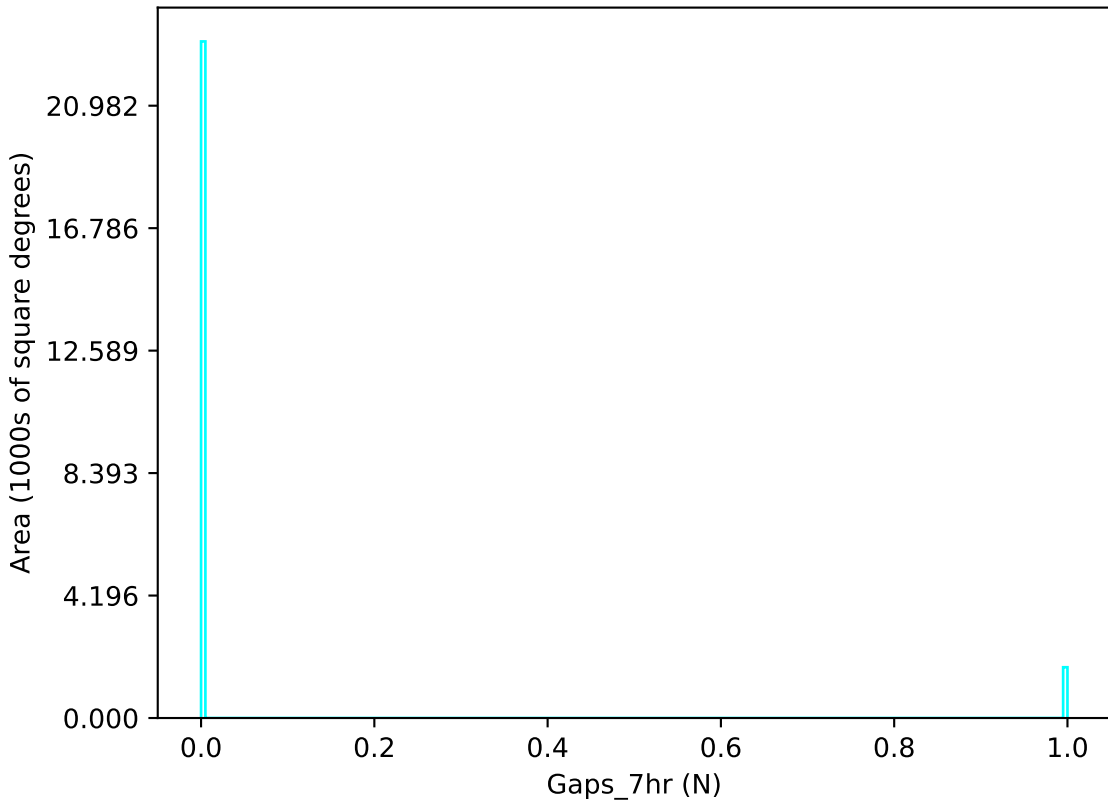
too_elab_r128_d3_giz_v3.4_10yrs u band: Gaps_7hr
