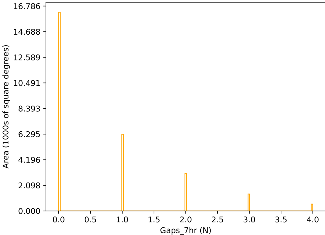
too_elab_r128_d3_giz_v3.4_10yrs r band: Gaps_7hr
