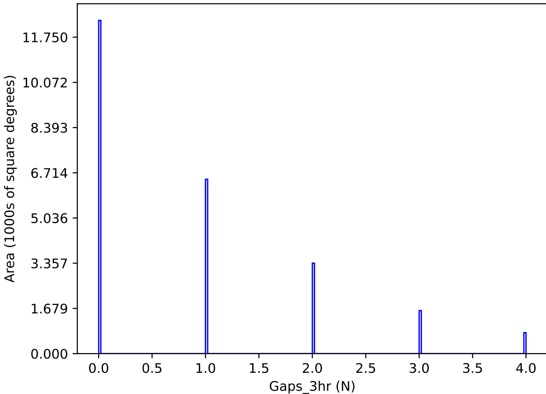
too_elab_r128_d3_giz_v3.4_10yrs y band: Gaps_3hr
