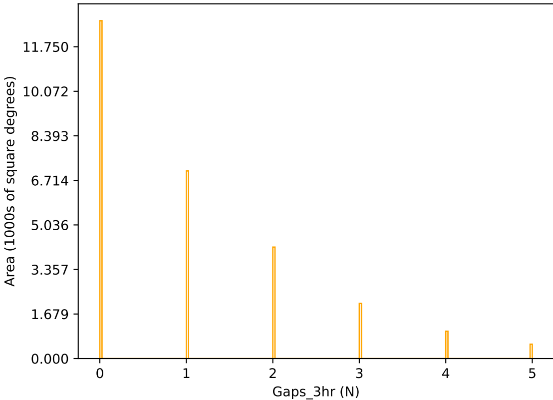
too_elab_r128_d3_giz_v3.4_10yrs r band: Gaps_3hr
