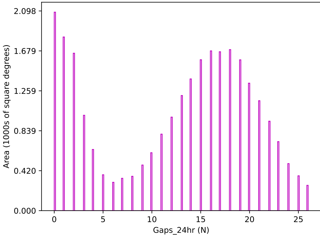
too_elab_r128_d3_giz_v3.4_10yrs z band: Gaps_24hr
