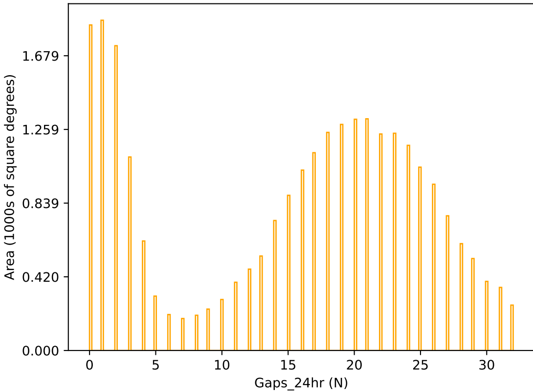
too_elab_r128_d3_giz_v3.4_10yrs r band: Gaps_24hr
