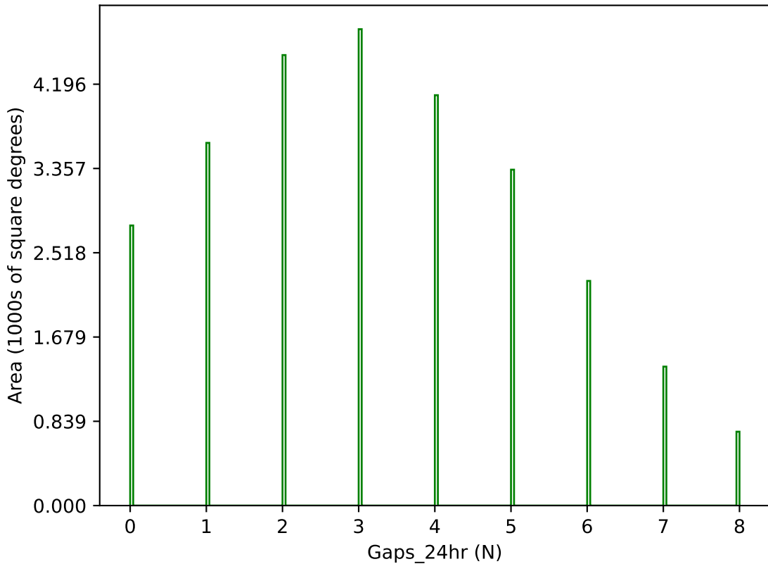
too_elab_r128_d3_giz_v3.4_10yrs g band: Gaps_24hr
