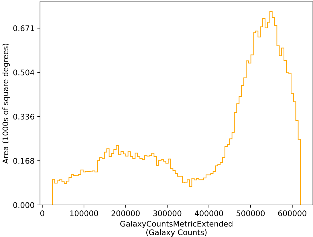
too_elab_r128_d3_giz_v3.4_10yrs r: GalaxyCountsMetricExtended
