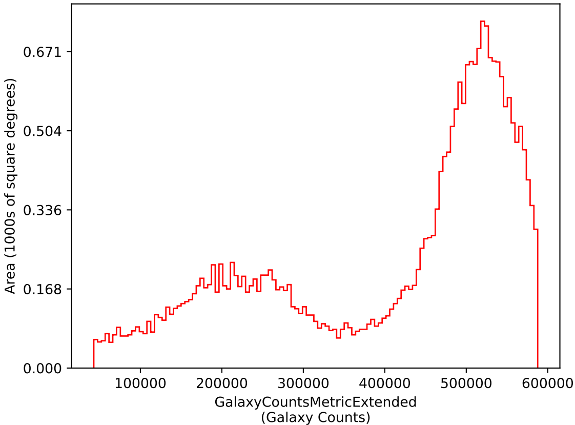
too_elab_r128_d3_giz_v3.4_10yrs i: GalaxyCountsMetricExtended
