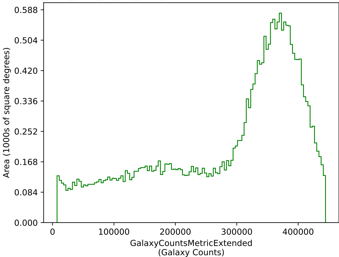
too_elab_r128_d3_giz_v3.4_10yrs g: GalaxyCountsMetricExtended
