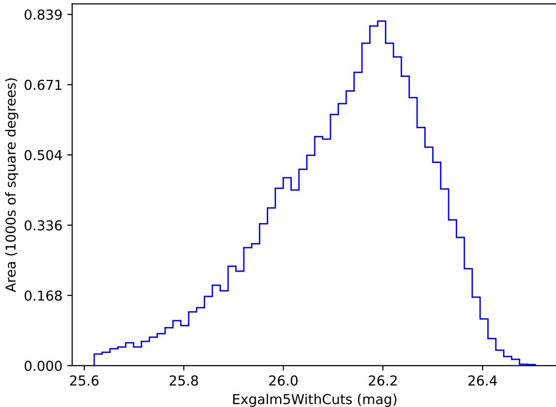
too_elab_r128_d3_giz_v3.4_10yrs i band non-DD year 6: ExgalM5WithCuts
