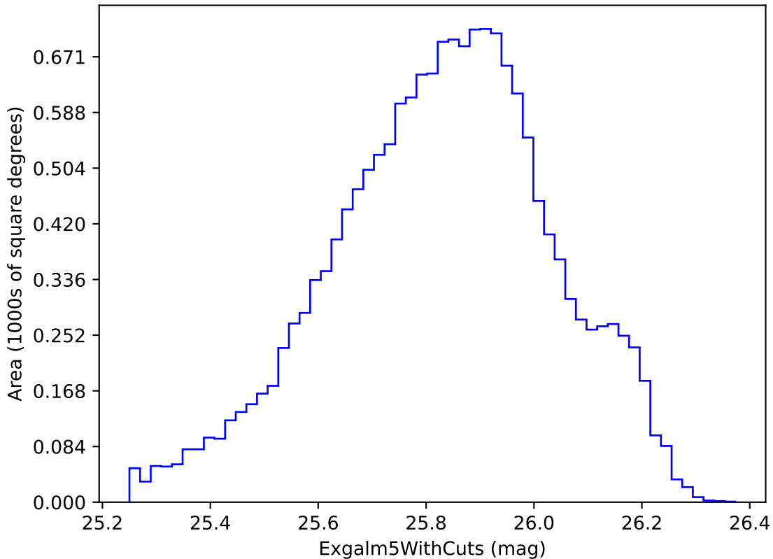
too_elab_r128_d3_giz_v3.4_10yrs i band non-DD year 3: ExgalM5WithCuts
