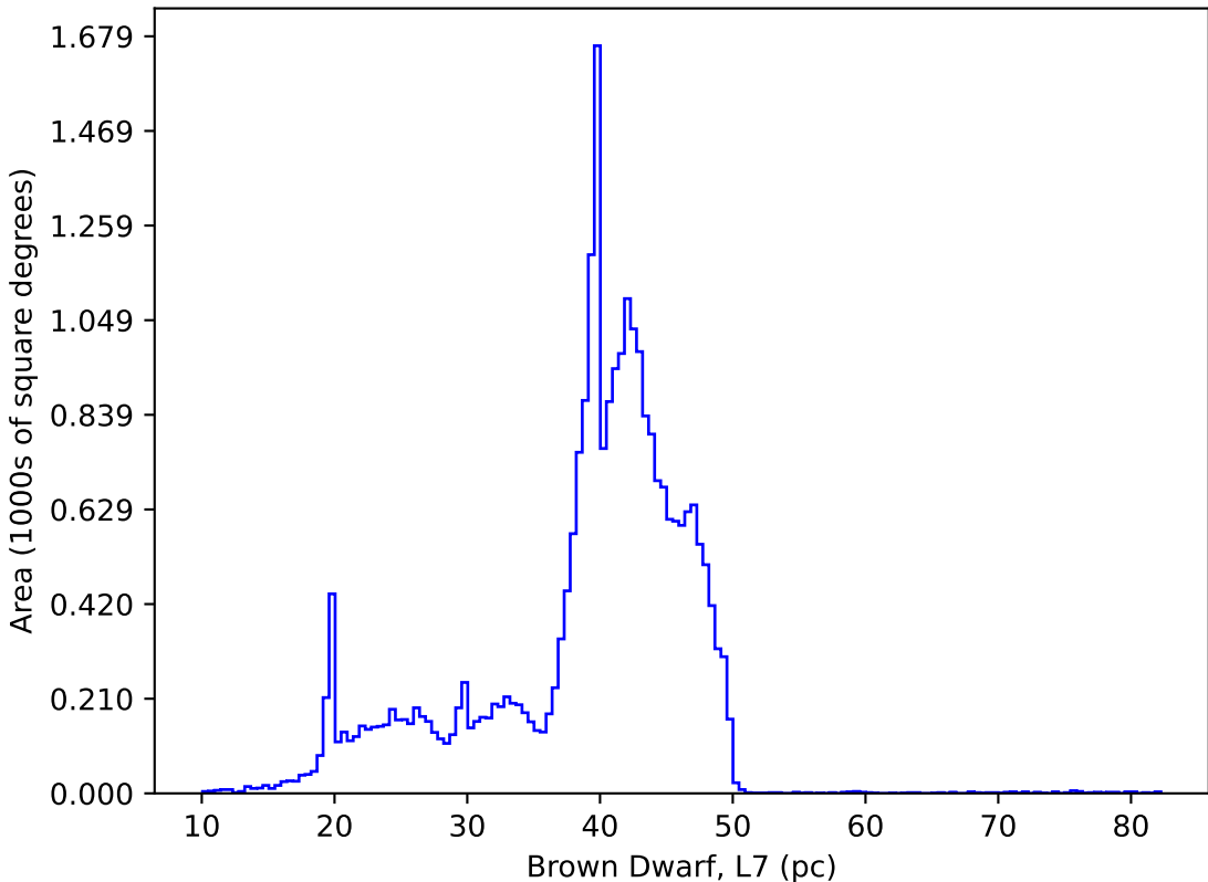
too_elab_r128_d3_giz_v3.4_10yrs : Brown Dwarf, L7
