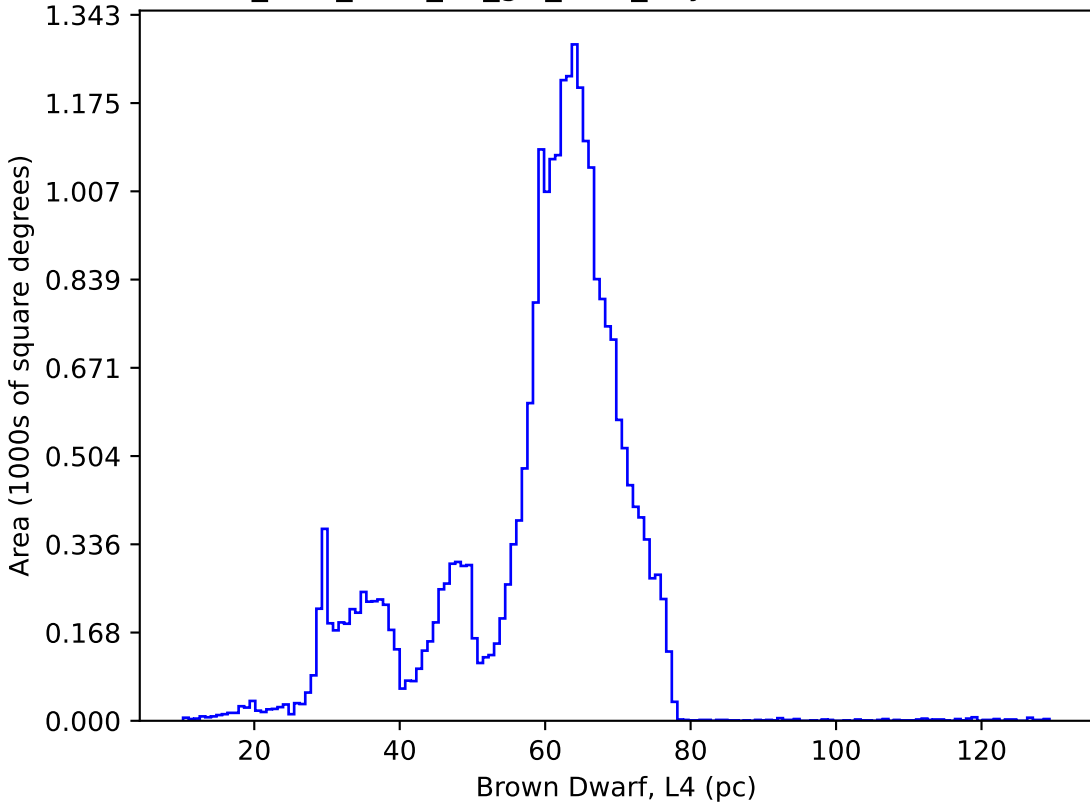
too_elab_r128_d3_giz_v3.4_10yrs : Brown Dwarf, L4
