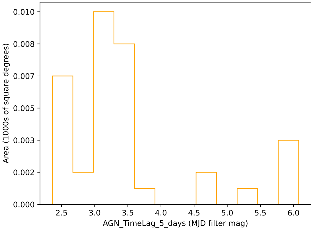
too_elab_r128_d3_giz_v3.4_10yrs r band: AGN_TimeLag_5_days
