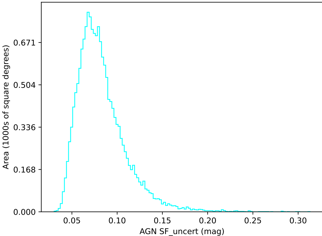
too_elab_r128_d3_giz_v3.4_10yrs u band: AGN SF_uncert
